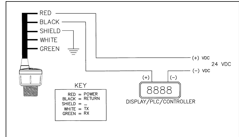
Typical Wiring Diagram Your WebCal Wiring Diagram may vary.
